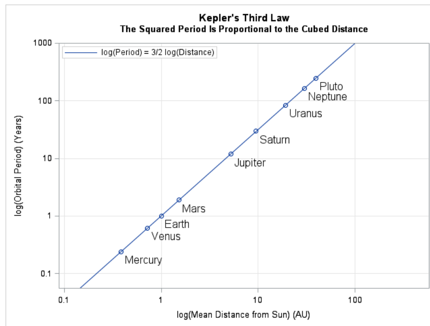
Kepler (planets)
