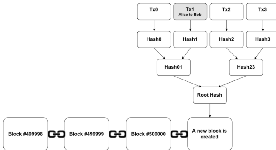
Fig. 6. Example of a Merkle Tree Structure (Source: Digital Asset Research)
